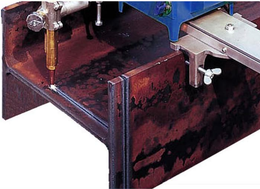
KC - 2 H Beam Gas Cutting Cutting Thickness 6 - 60 mm Cutting W x H : 800 x 400 mm
