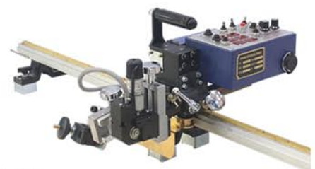
KC - 300 Welding Carriage Continuous and Interval Welding Travel Speed : 30 - 800 mm/min
