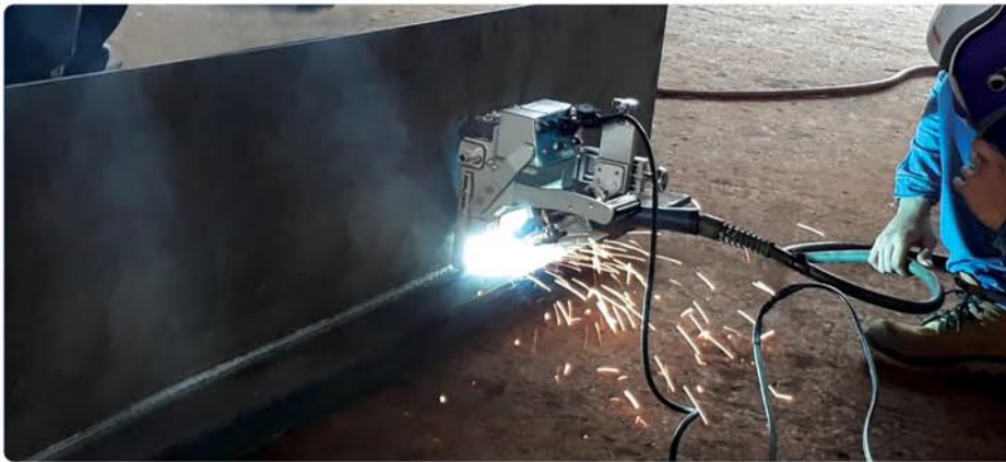
KC - 100 Welding Carriage Continuous Welding Travel Speed : 150 - 1.500 mm/min
