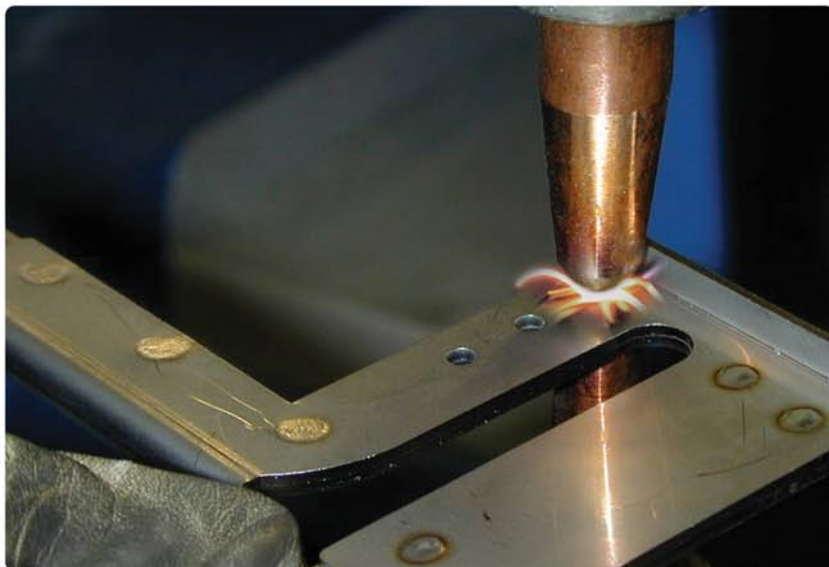
DAICHI Japan Spot Welding
